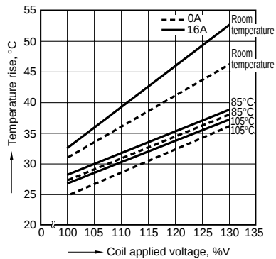
2. Coil temperature rise
